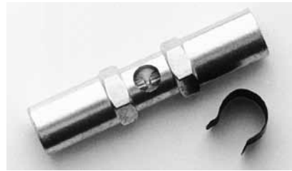
Brake Cable Coupling and Oiler, Cad Plated Cad plated solid brass coupling is an exact reproduction of the original Harley design and includes the dust cover. Coupling OEM 4142-30. Fits all models H.D. 1930-38.
