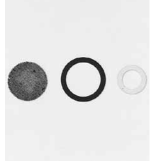
Gas Strainer Rebuild Kit OEM 3627-39 screen, OEM 3613-39 gasket and body to carburetor gasket to rebuild in line style gas strainer used on all Twins 1939-1941. Stock No. 9731-3
